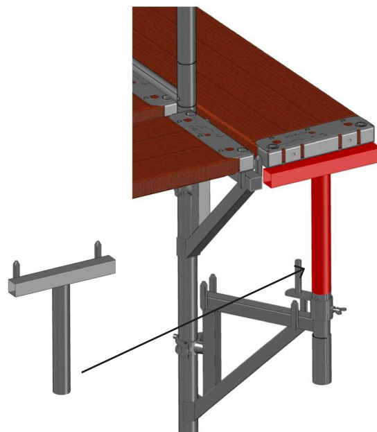
example of use with wooden decks plettac SL
